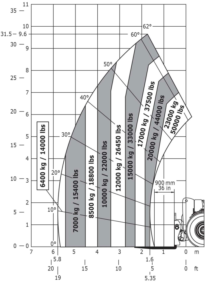
Machine on tyres with forks - CoG 900 mm
